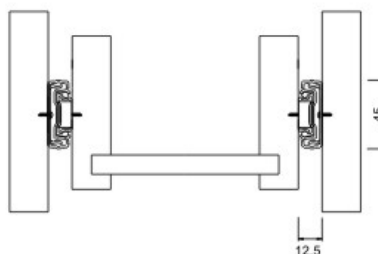
Side mounting 45mm ball bearing slides Load Capacity: 45kgs
