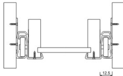
Clamp On type Self closing drawer slides Tolerance of installation: 1/2"(12.5mm)
