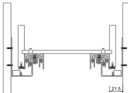
Peg locking Soft closing concealed slides Full extension
