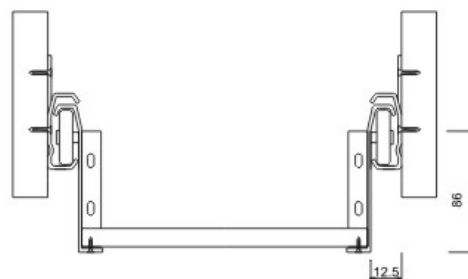
Metal side type Self closing drawer slides Height: 86mm, 118mm, 150mm
