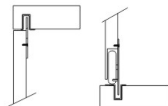
Sliding door roller Side mounted Material: Nylon
