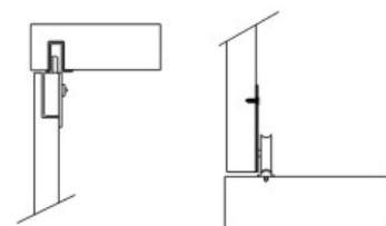
Sliding door roller Side mounted Material: Nylon
