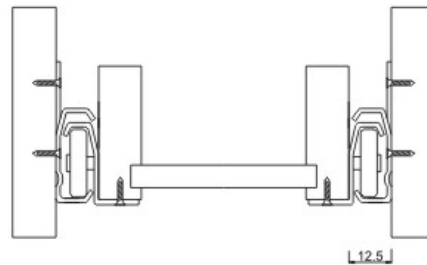
FGV type Self closing drawer slides Tolerance of installation: 1/2"(12.5mm)
