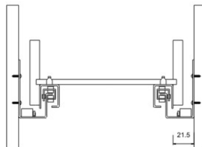
Handle locking type Soft closing Concealed slides 3/4" extension and invisible bottom mounting
