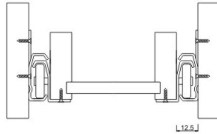
Blum type Self closing drawer slides Tolerance of installation: 1/2"(12.5mm)
