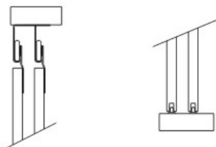
Sliding door roller Hang on type for 2 doors Load capacity: 45kgs
