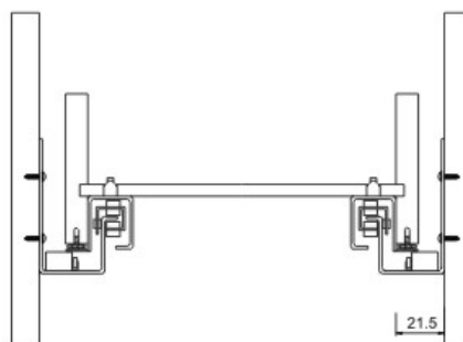
Peg locking type Soft closing Concealed slides 3/4" extension
