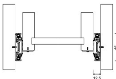
Bottom mounting 45mm ball bearing slides Load Capacity: 45kgs
