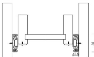
Bottom mounting 35mm ball bearing slides Load Capacity: 30kgs
