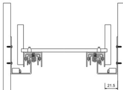
Handle locking type Concealed slides Full extension
