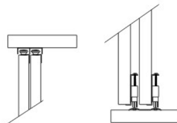
Sliding door roller Light duty Load capacity: 25kgs
