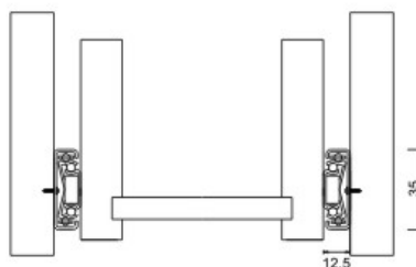
Soft closing 35mm Ball bearing slides Load capacity: 30kgs
